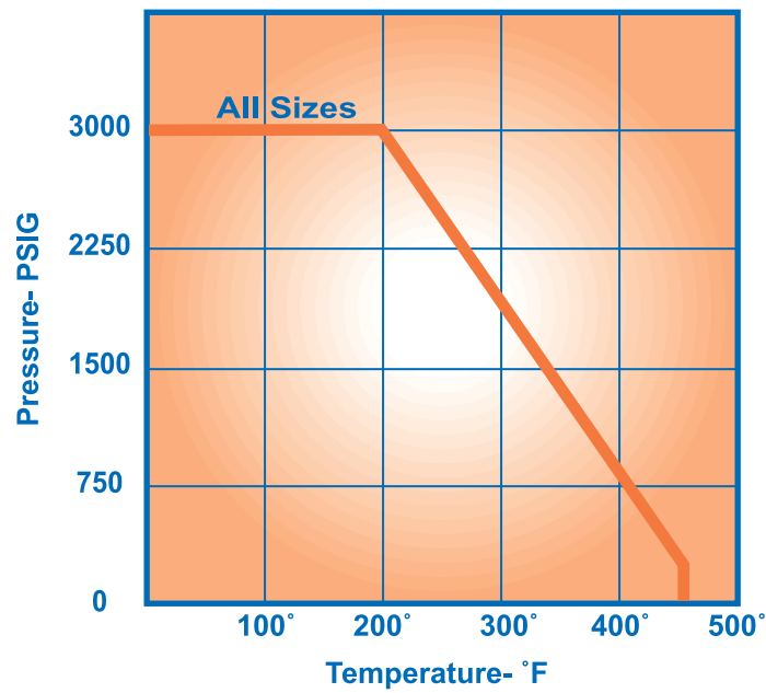
PEEK Seats
