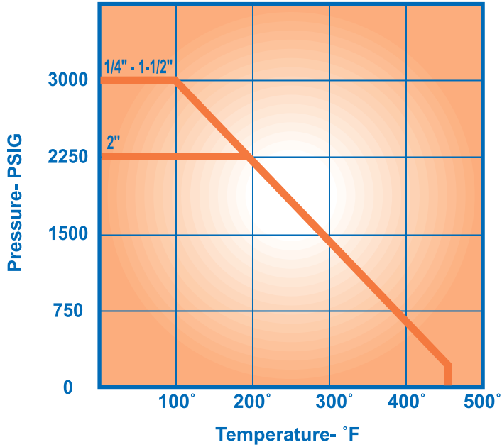
RTFE Seats
